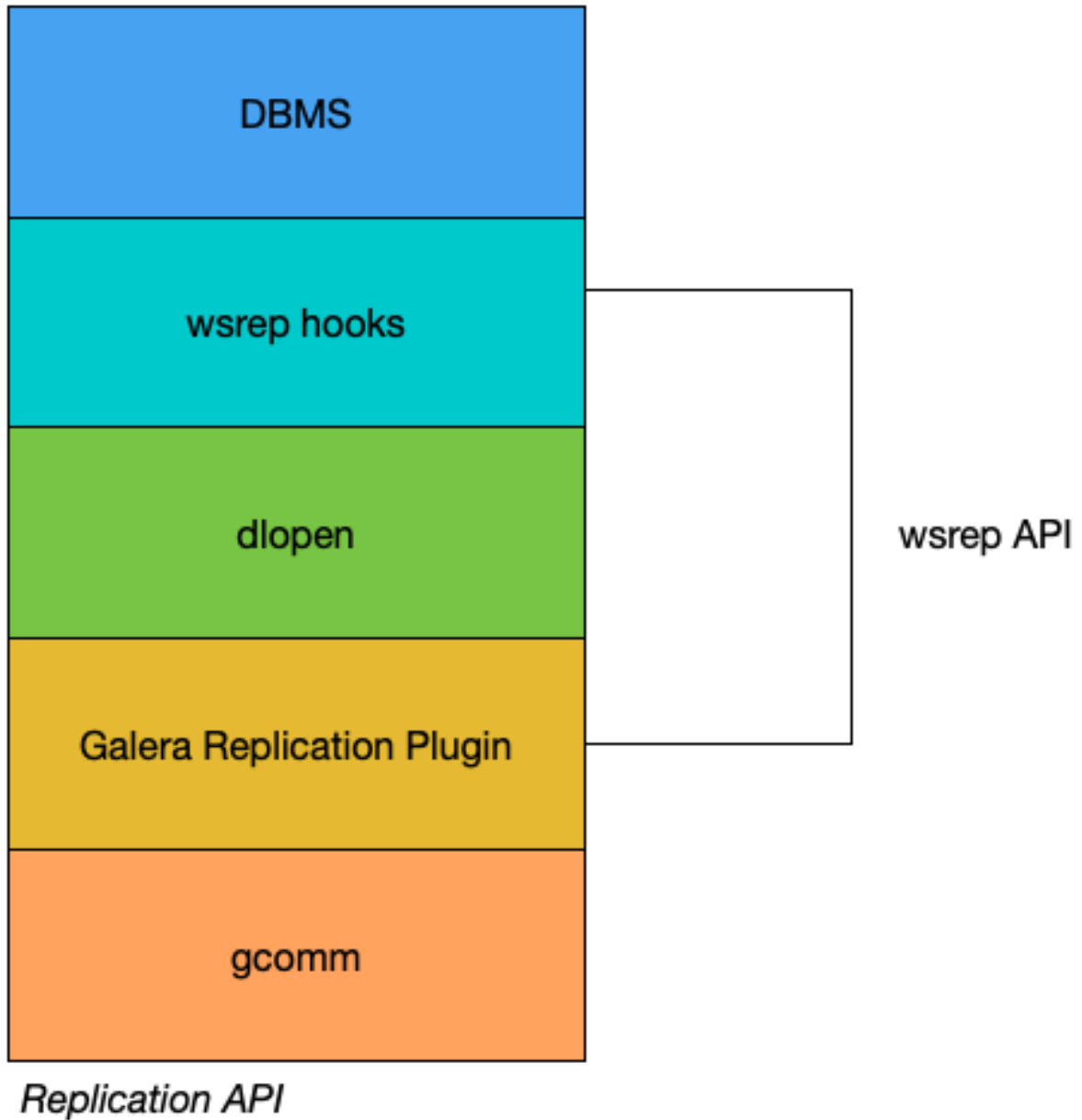
Fig. 4: Replication API
