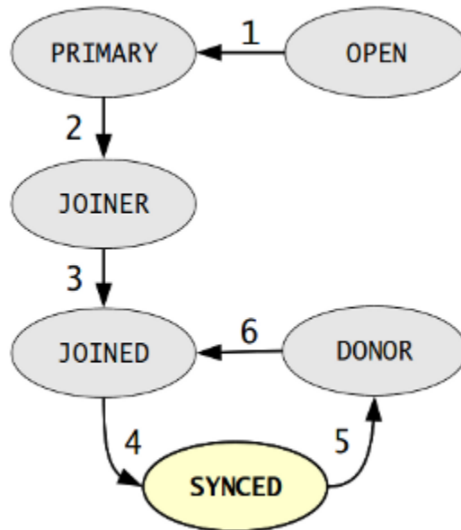
Fig. 5: Galera Cluster Node State Changes
