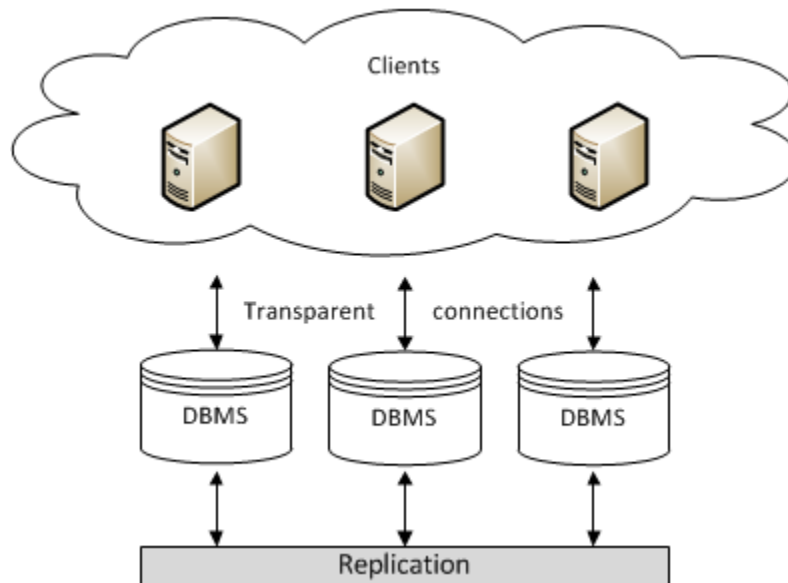
Fig. 2: Multi-master Replication
