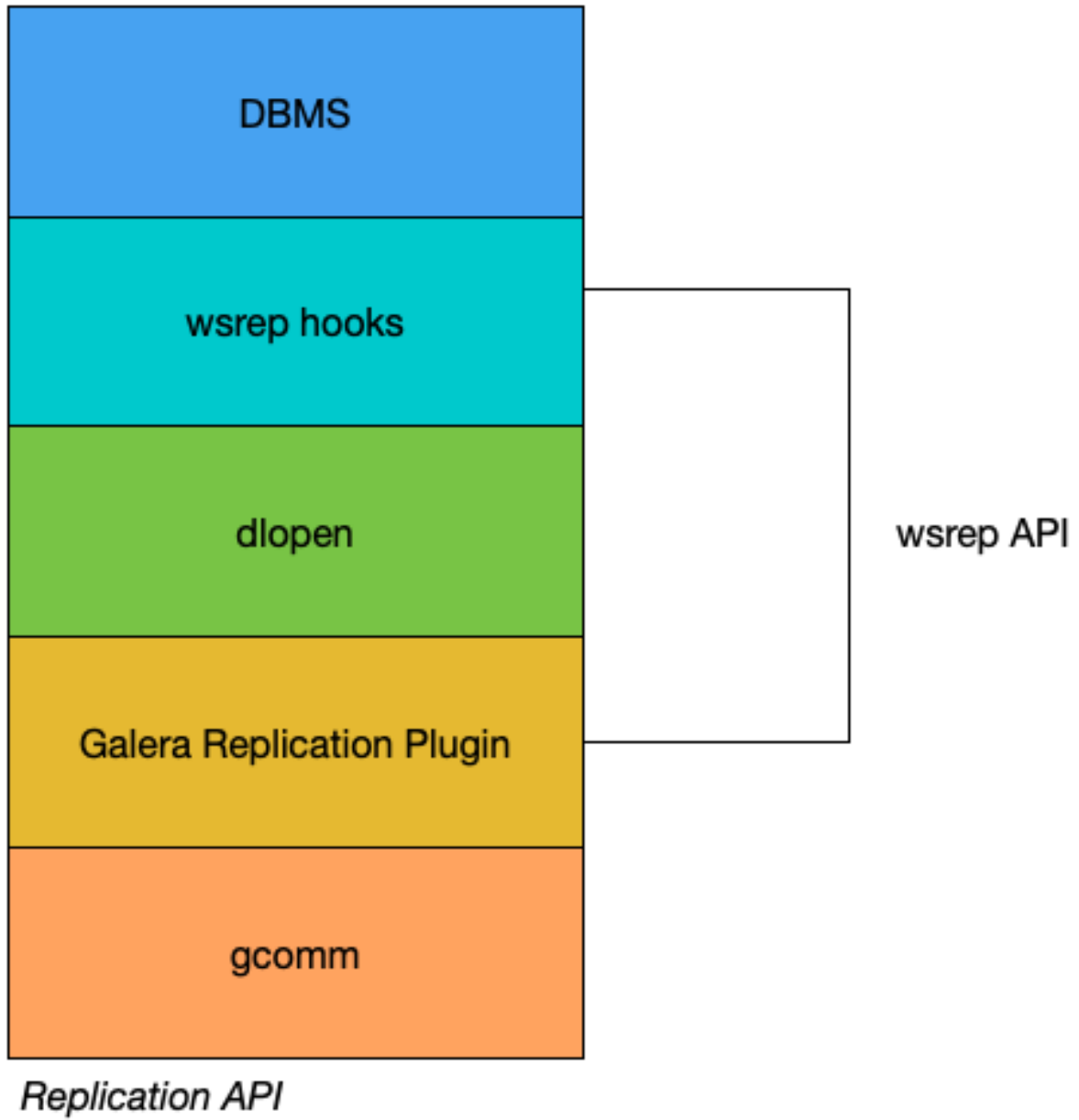
Fig. 4: Replication API
