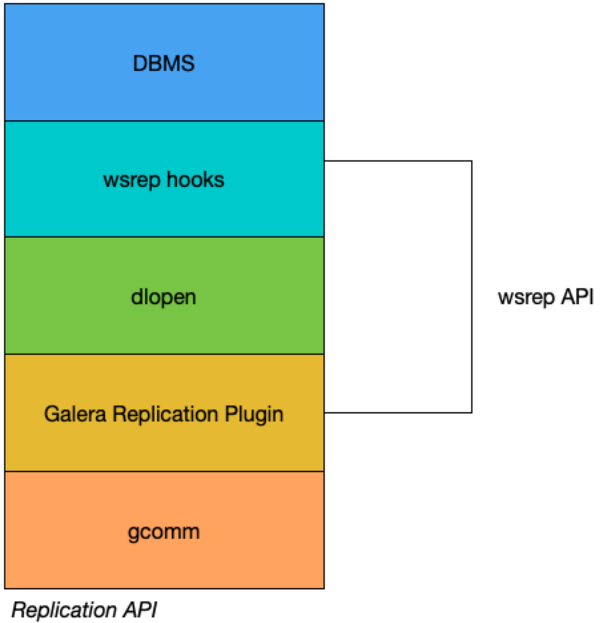
Fig. 4: Replication API
